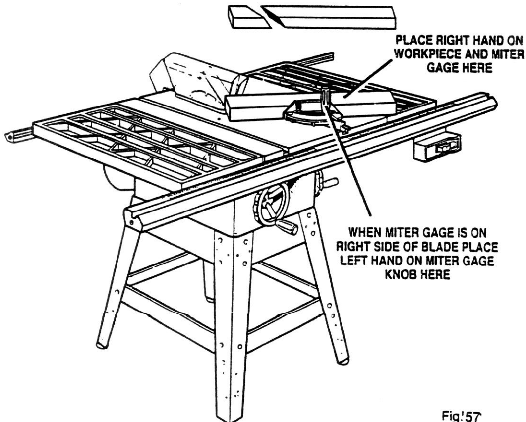
COMPOUND (BEVEL) MITER CUT
